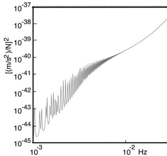
Figure 5. The function E(f) describing the Earth normal excitation by a time varying vertical point force at the Earth's surface versus frequency f .
