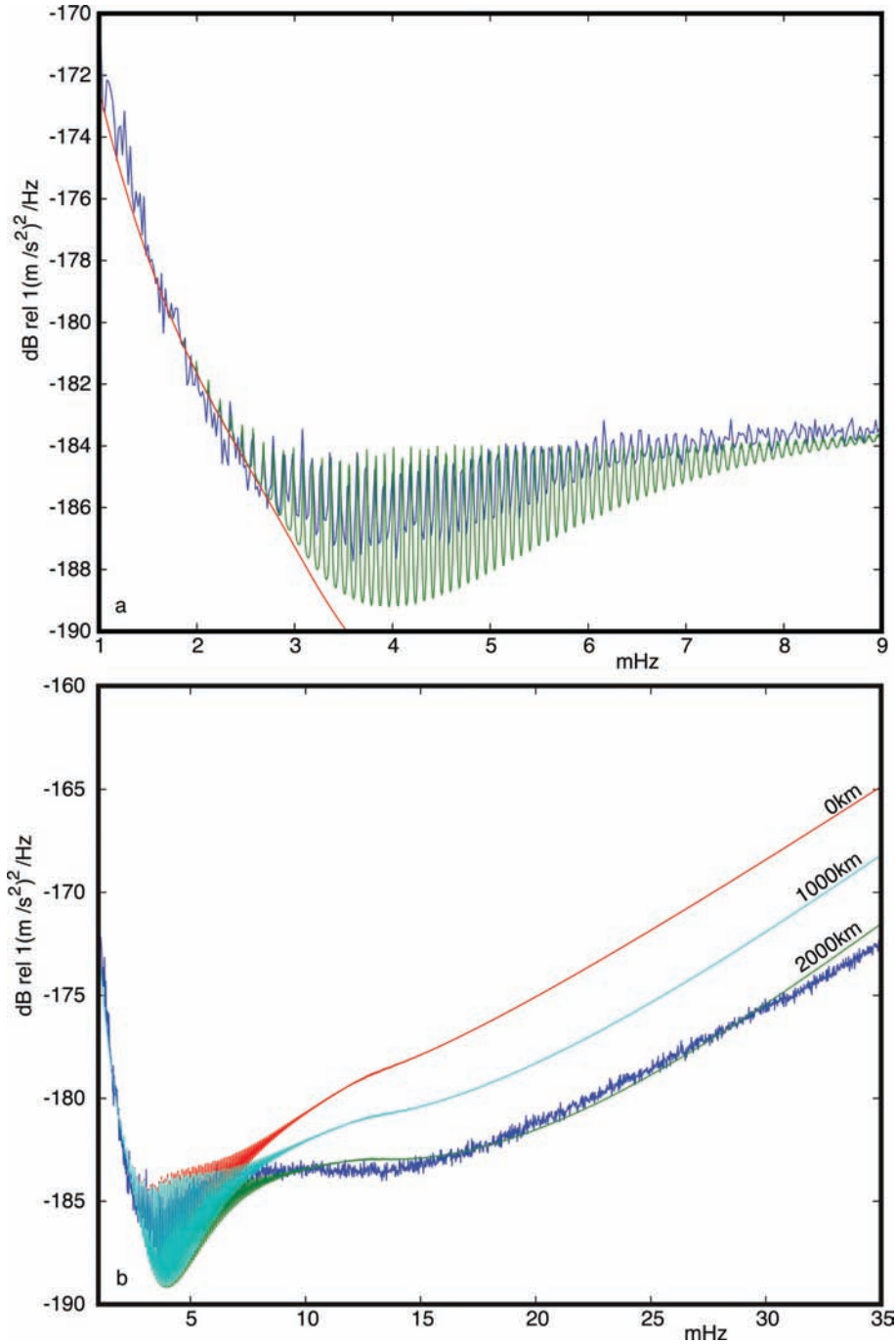
Figure 8. Same as Fig. 4 except here comparing the vertical acceleration spectrum resulting from infragravity waves interacting over the deep ocean basins. (a) assumes the distance from the nearest source region to the site is 2000 km. (b) same as (a), except showing the predicted spectrum for different distances from the receiver to the nearest energetic source.
