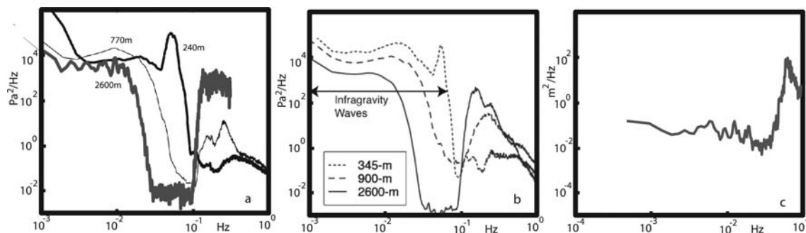
Figure 3. (a) Pressure spectra from three water depths in the Northern Pacific. The two shallow sites are from near San Diego, the deep site is from the East Pacific Rise near 10^{\circ}\text{N} . (b) Pressure spectra from three water depths in the Northern Atlantic near the Faroes Islands (Crawford et al. 2005). (c) Energetic wave height spectra from offshore of Florida (redrawn from Herbers 2006).
