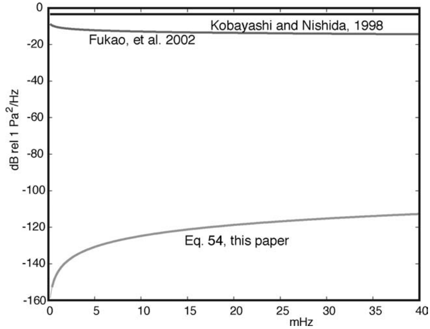
Figure 10. Estimates of the component of the surface pressure spectra under atmospheric turbulence at phase velocity high enough to be relevant to driving the Earth’s hum as inferred from three models of turbulence. A label below each curve notes the relevant reference. The two previous models greatly overestimated the long wavelength component of atmospheric turbulence.
