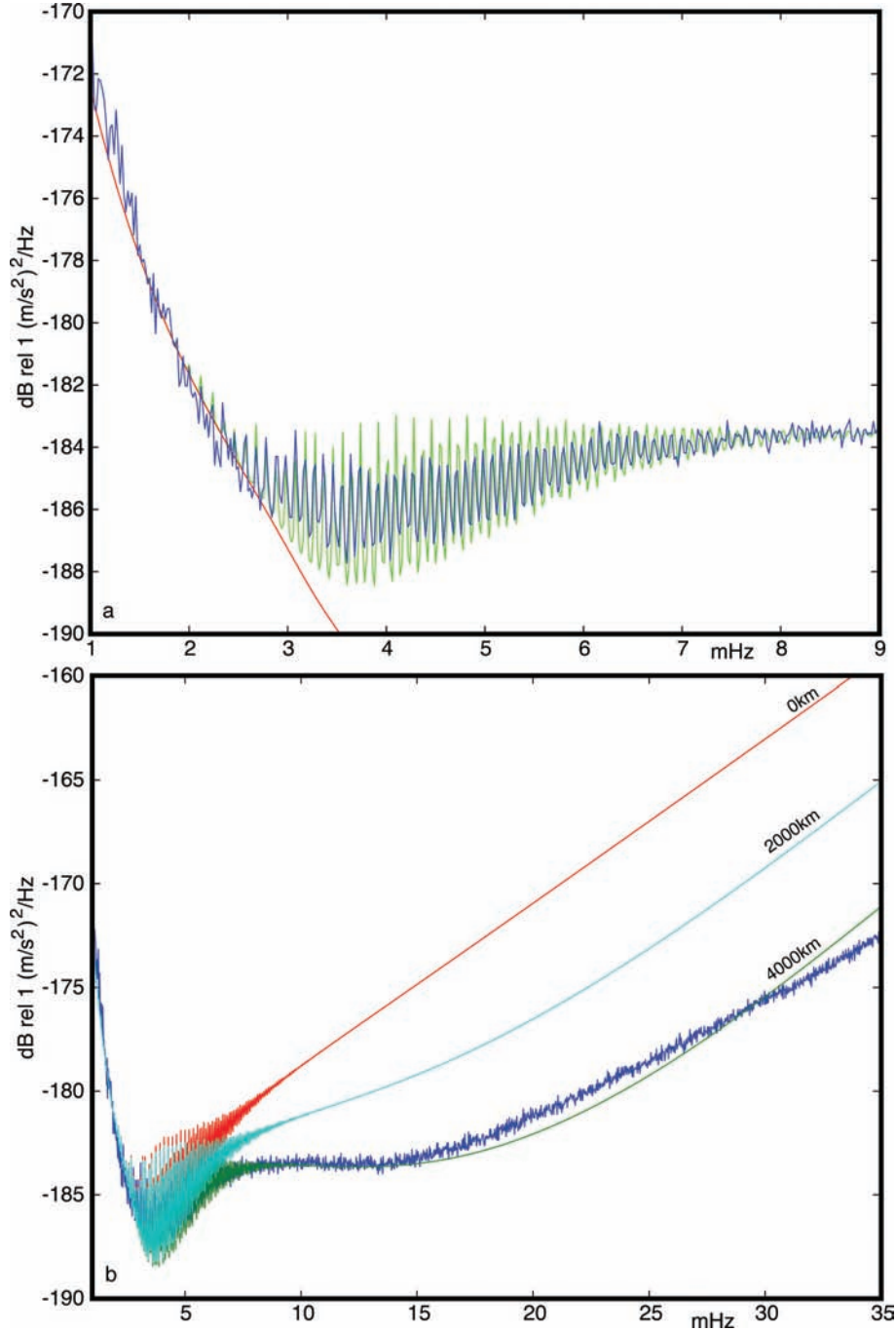
Figure 4. (a) Spectrum predicted from the interaction of energetic infragravity waves over the continental shelf (green) compared with observations of the Earth's hum derived from selected spectra from quiet sites (blue line, Berger et al. 2004). A model for the spectra of the time varying gravitational attraction of the atmosphere has been added to the model (red line). Fit assumes a distance of 4000 km from nearest sources to the receiver. (b) Same as (a), except shows predicted spectra for different distances from the receiver to the nearest energetic source.
