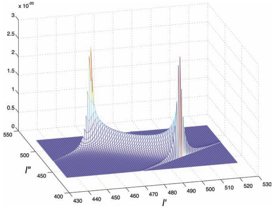
Figure 6. The resulting forcing of Earth normal modes of order L = 40 , by the interaction of two infragravity wave modes of order l' and l'' . For any pair l', l'' , the forcing occurs at a frequency: \omega = (l' + l'')\Delta s .
