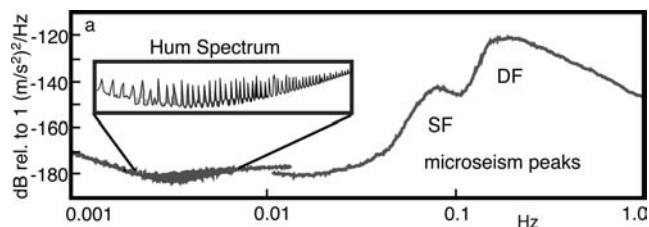
Figure 1. Vertical Acceleration spectrum from a quiet site (BFO) redrawn from figure by R. Widmer-Schmidvig. Insert: expanded view showing resonance peaks associated with earth normal modes.
