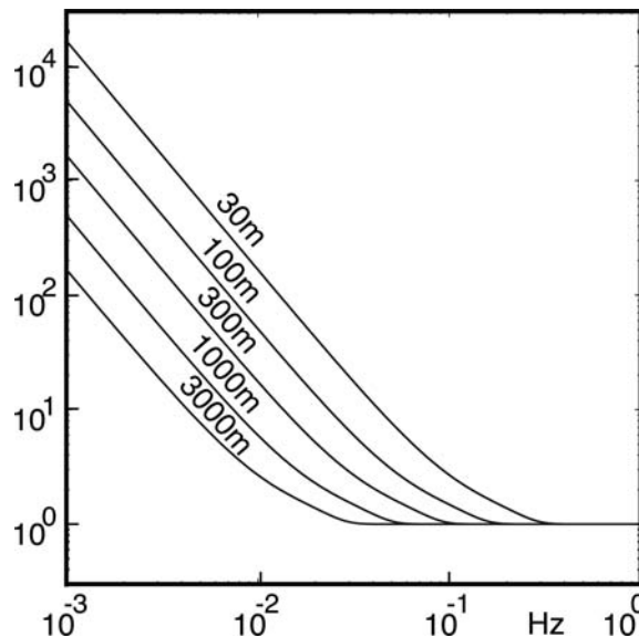
Figure 2. The function G(f, H) describing the relative strength of non-linear wave interaction is shown for five depths H versus frequency f .
