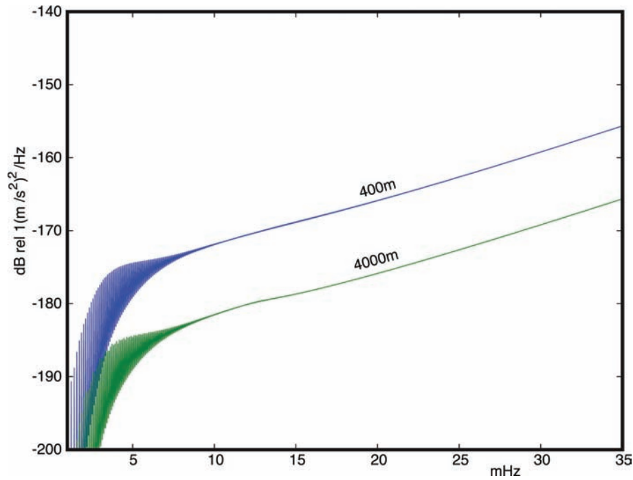
Figure 7. Estimates of the vertical acceleration spectrum that results from Earth seismic normal modes driven by the interaction of infragravity waves over the ocean basins predicted for two different water depths. The reciprocal dependence of the spectrum on water depth is the same as found for the continental shelf result (Fig. 2).
