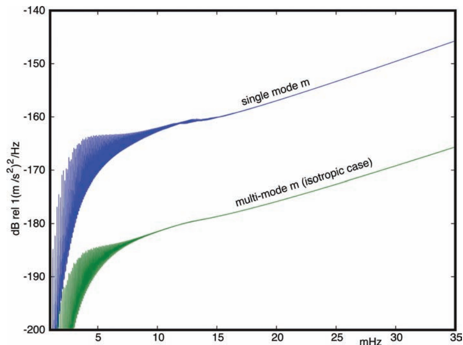
Figure 9. A comparison of the predicted vertical acceleration spectrum resulting from infragravity waves interacting over the ocean basins, but making two different assumptions about the distribution of energy between harmonics. The single mode curve assumes all of the energy is in a single (zonal) mode m = 0 . The multimode curve assumes energy is evenly partitioned between modes m .
